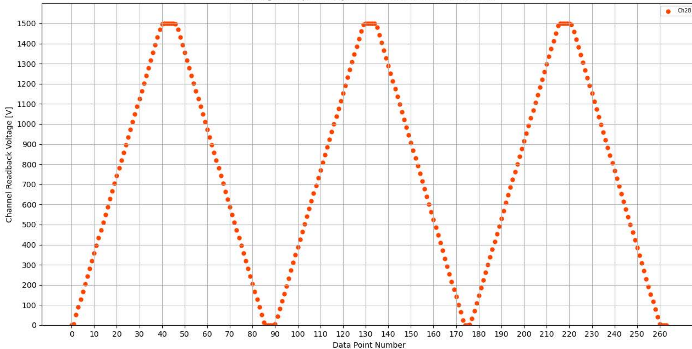
Voltage Ramp Test (Python) Bd #304, Slot #8, Ch #28
