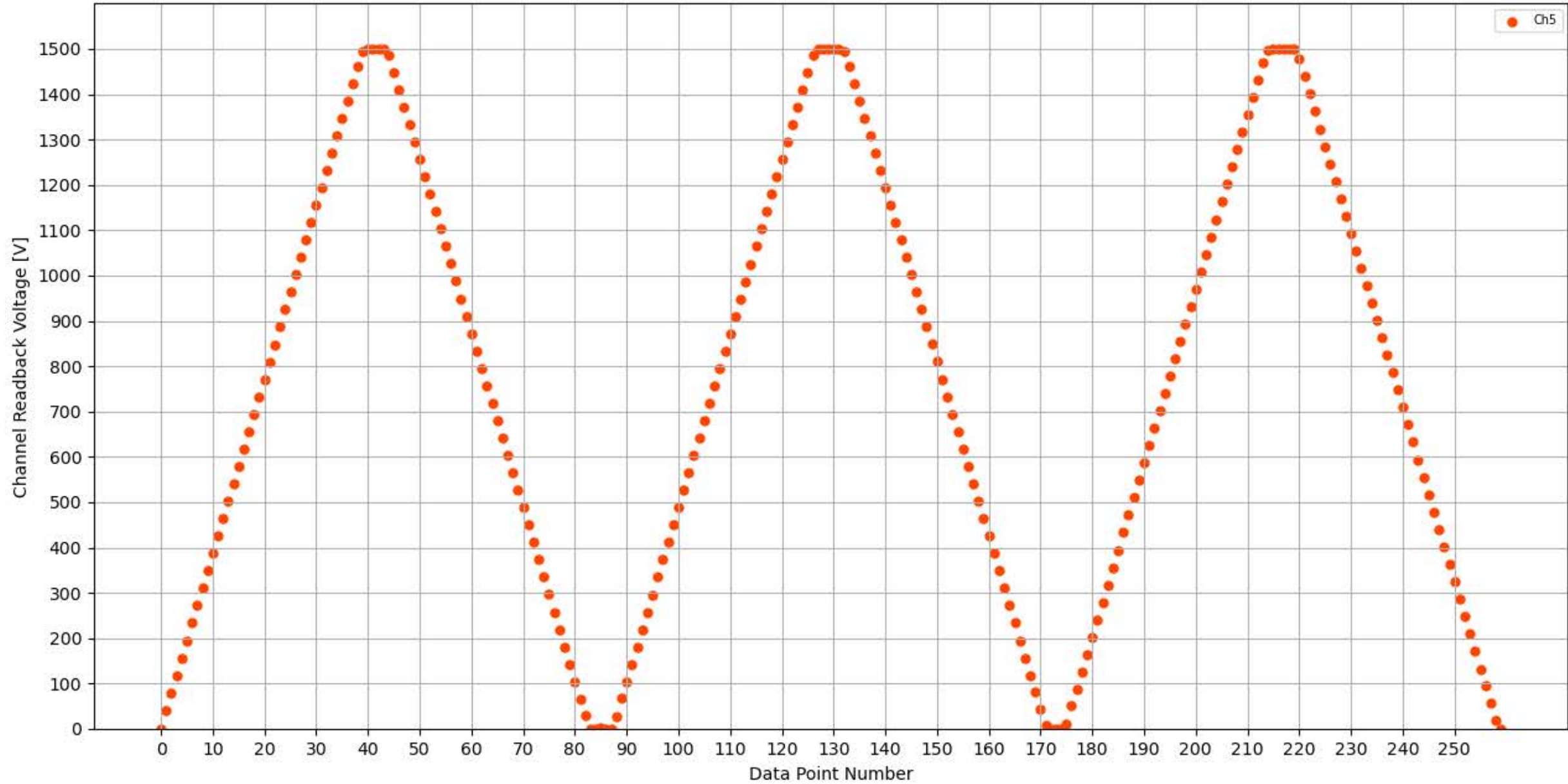
Voltage Ramp Test (Python) Bd #304, Slot #8, Ch #5
