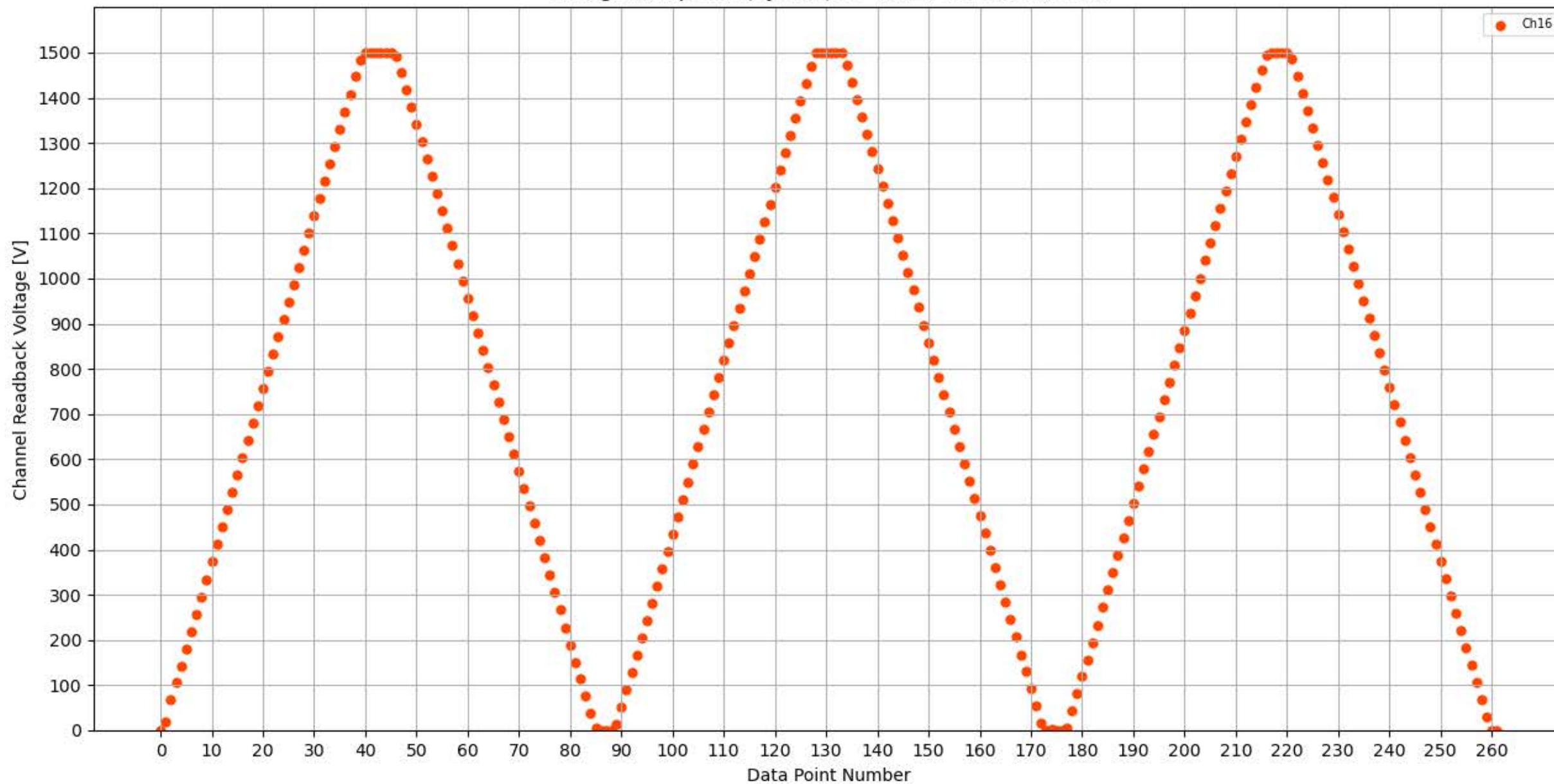
Voltage Ramp Test (Python) Bd #304, Slot #8, Ch #16
