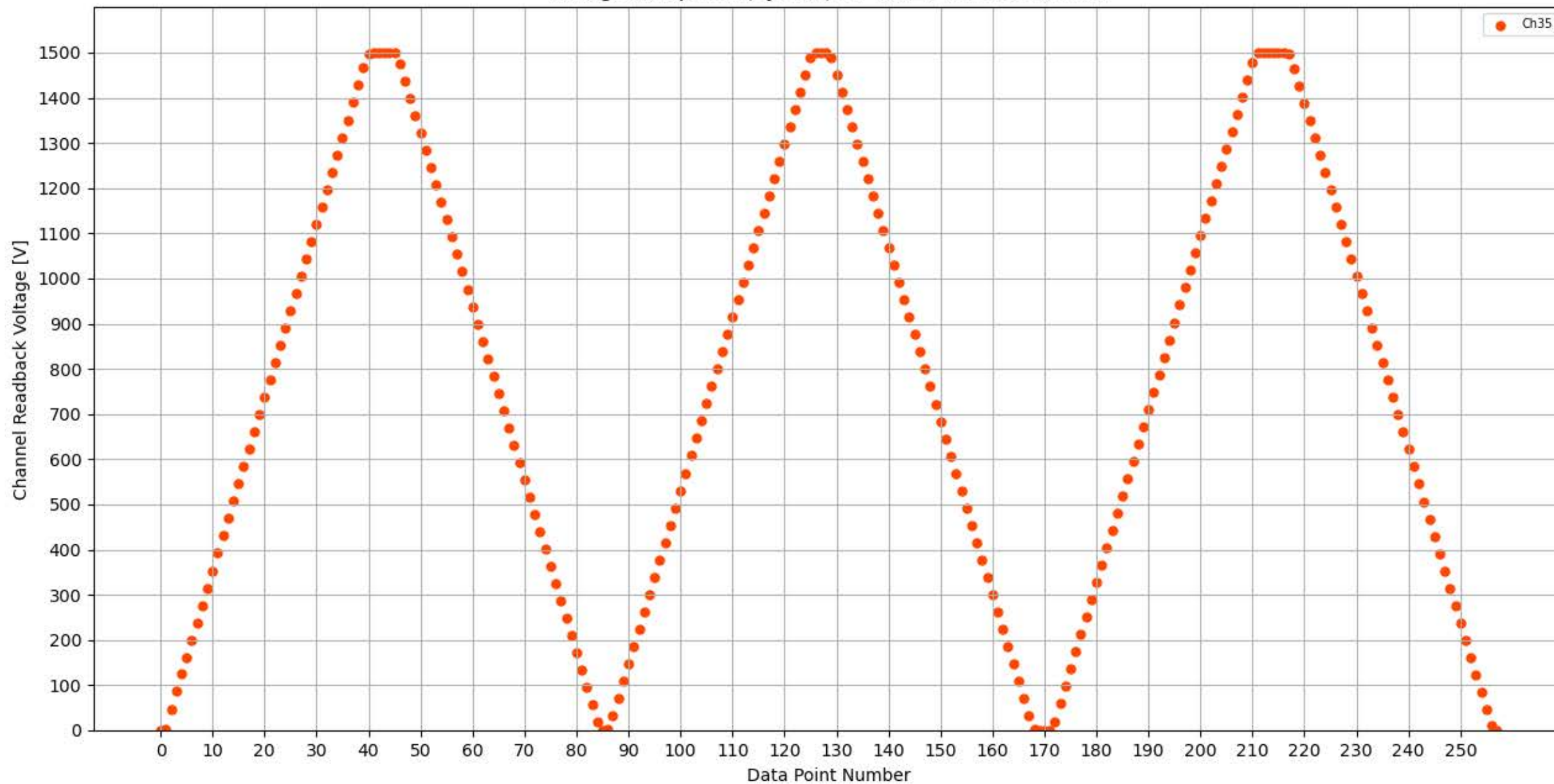
Voltage Ramp Test (Python) Bd #304, Slot #8, Ch #35
