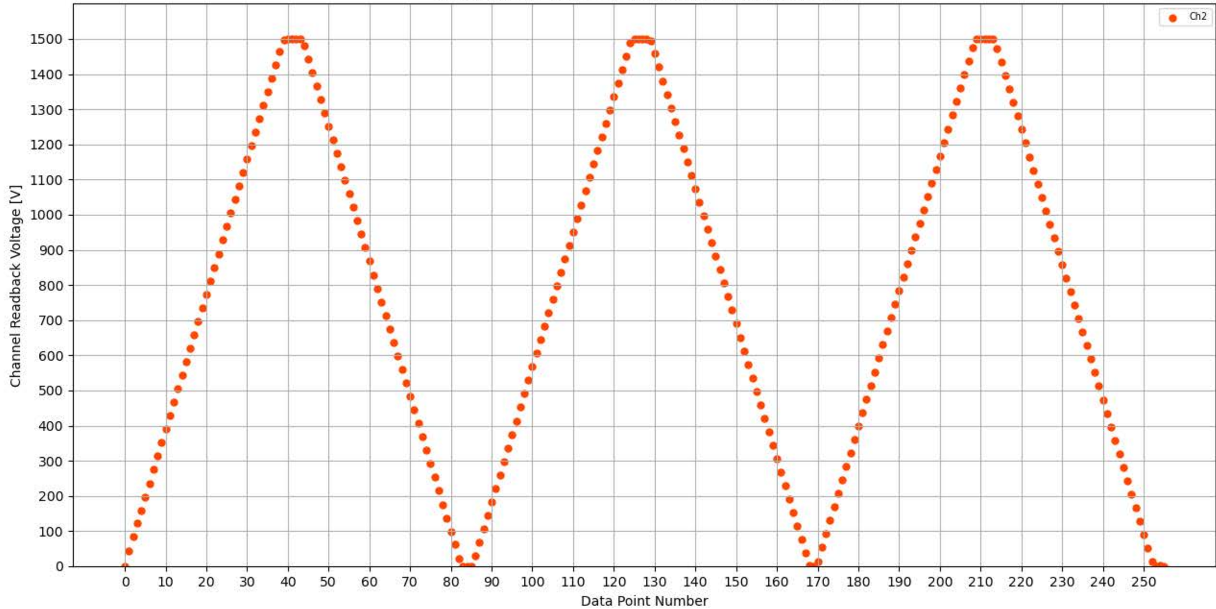
Voltage Ramp Test (Python) Bd #304, Slot #8, Ch #2
