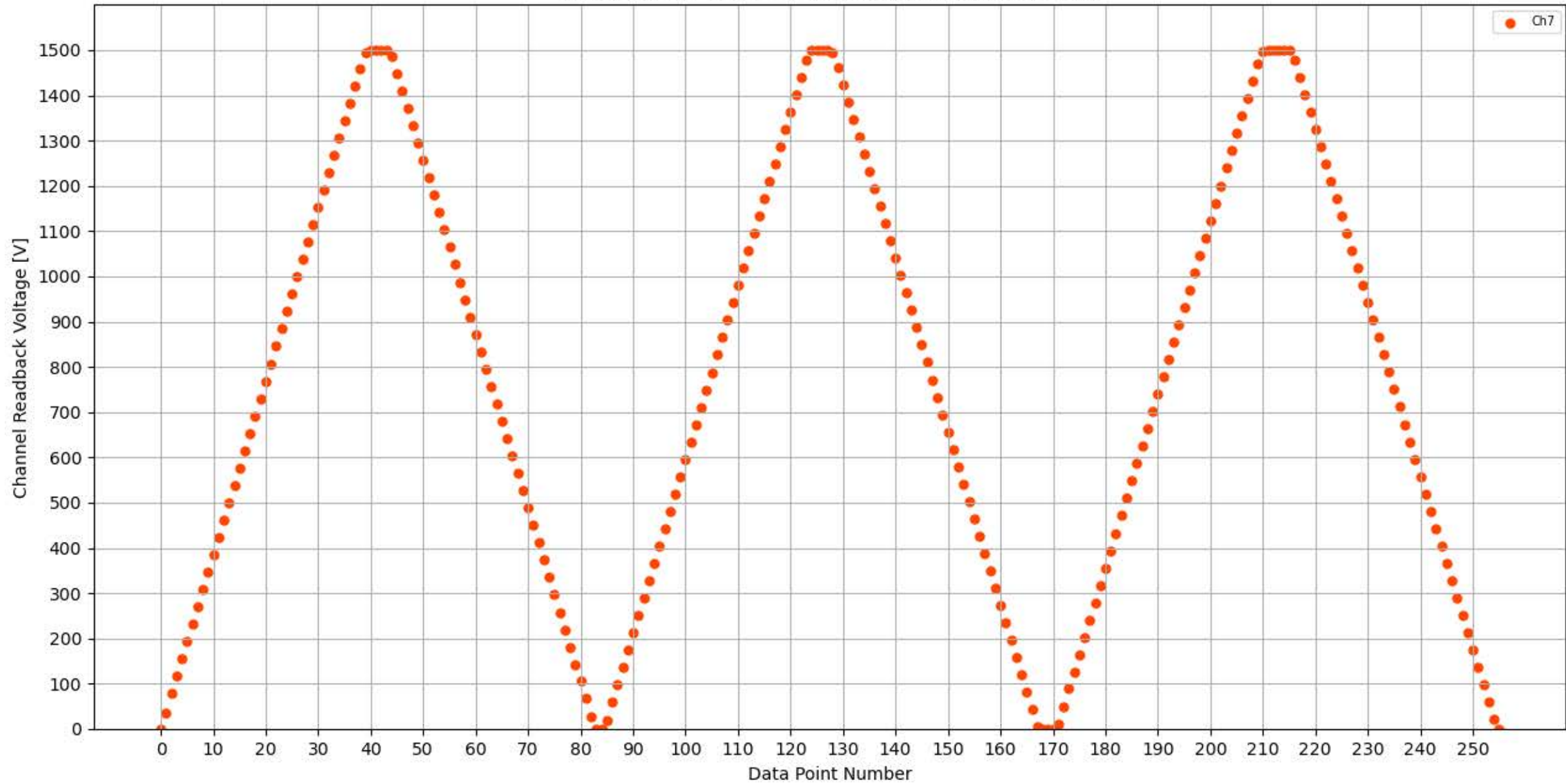
Voltage Ramp Test (Python) Bd #304, Slot #8, Ch #7
