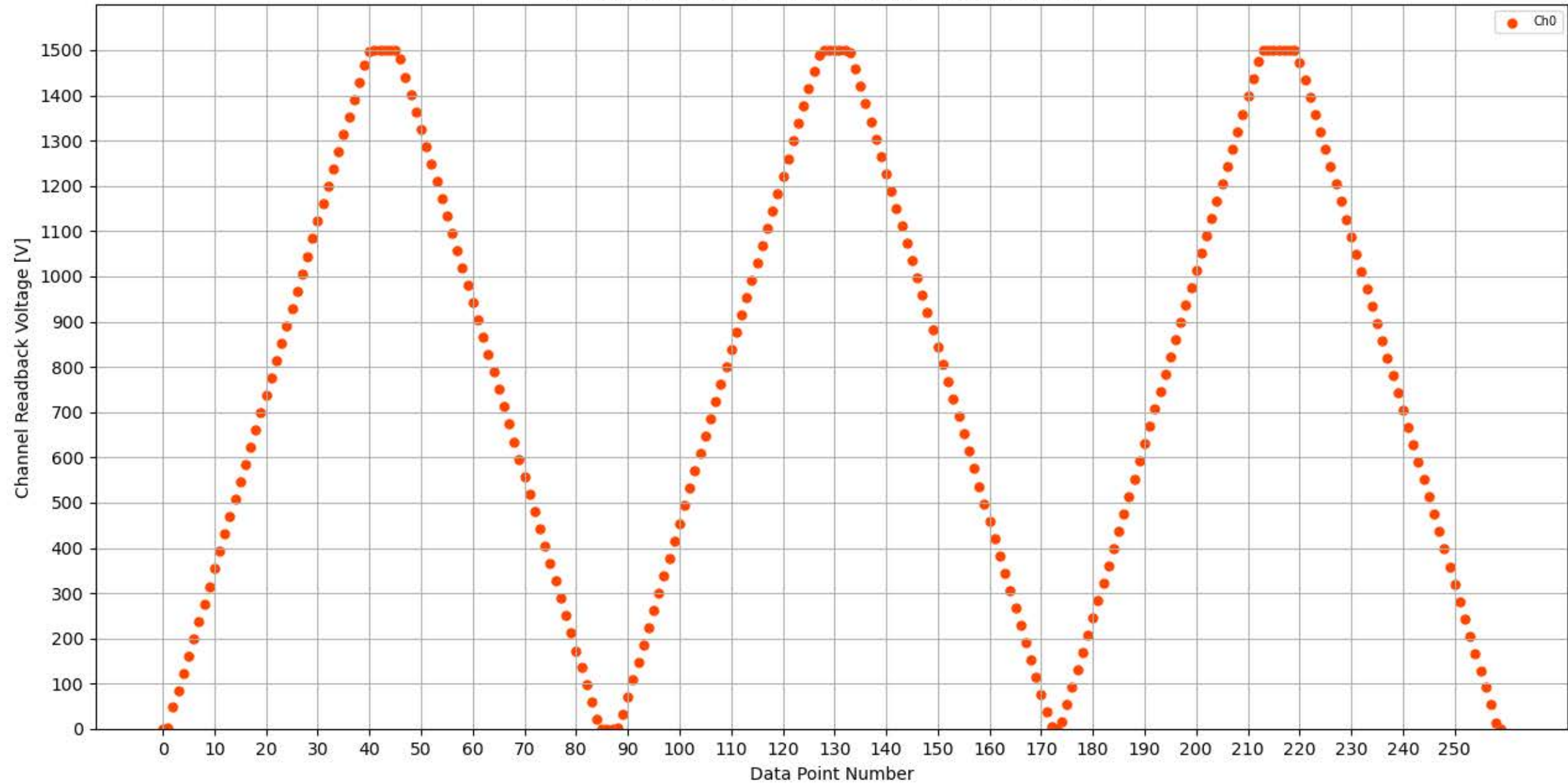
Voltage Ramp Test (Python) Bd #304, Slot #8, Ch #0
