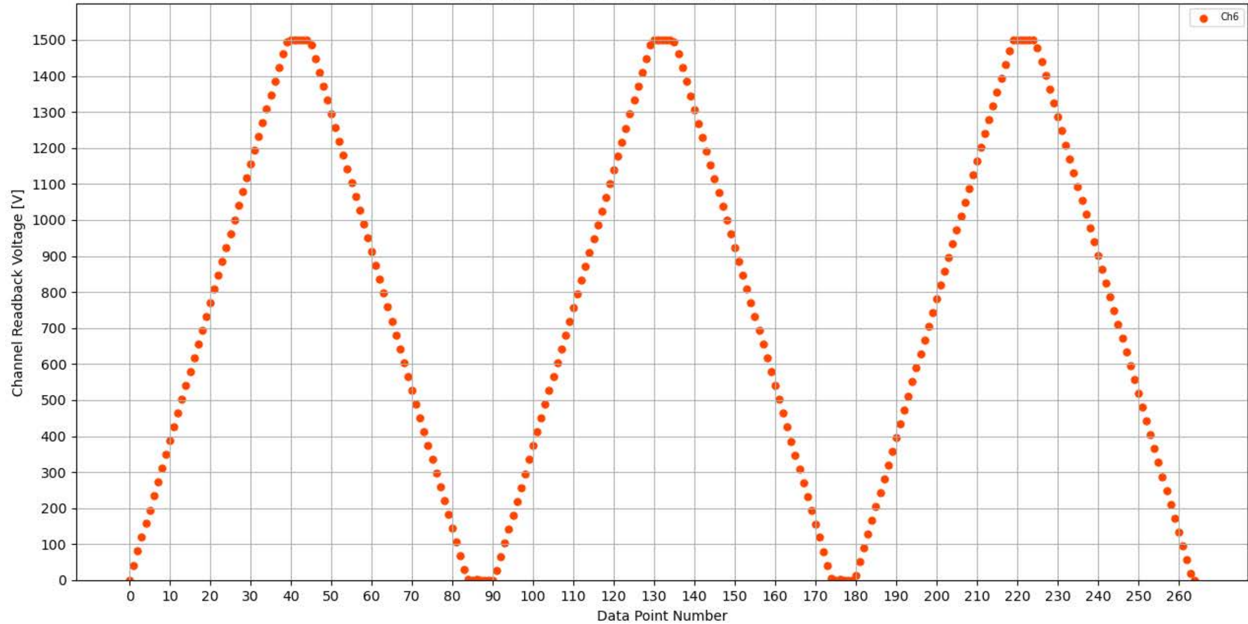
Voltage Ramp Test (Python) Bd #304, Slot #8, Ch #6
