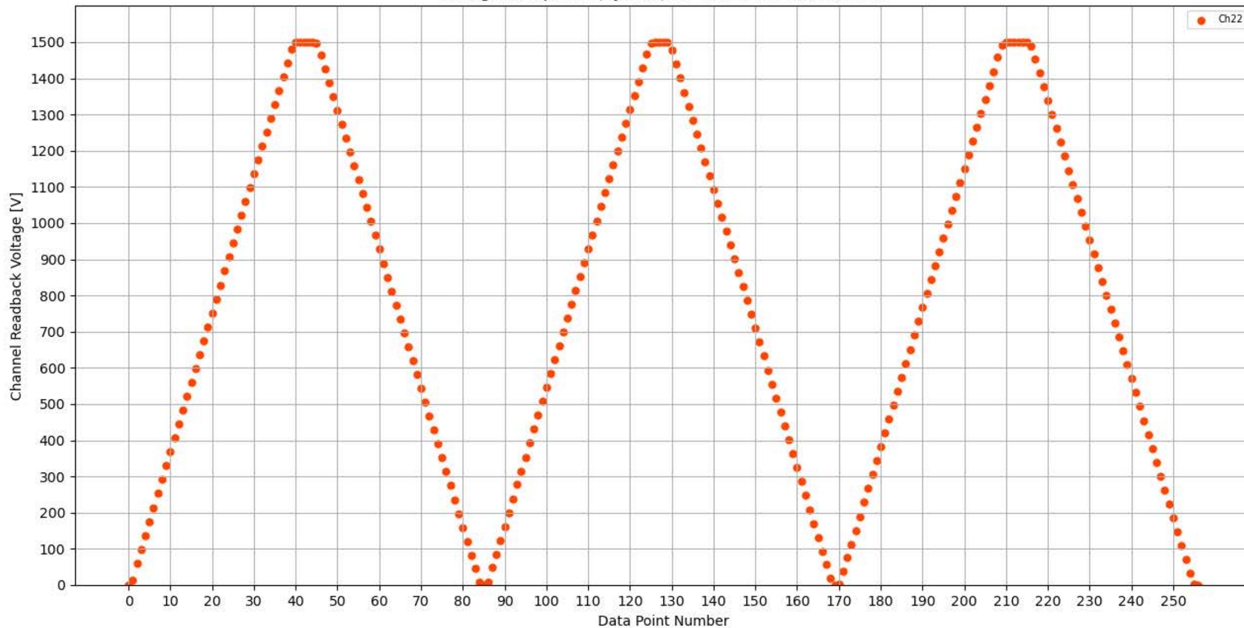
Voltage Ramp Test (Python) Bd #304, Slot #8, Ch #22
