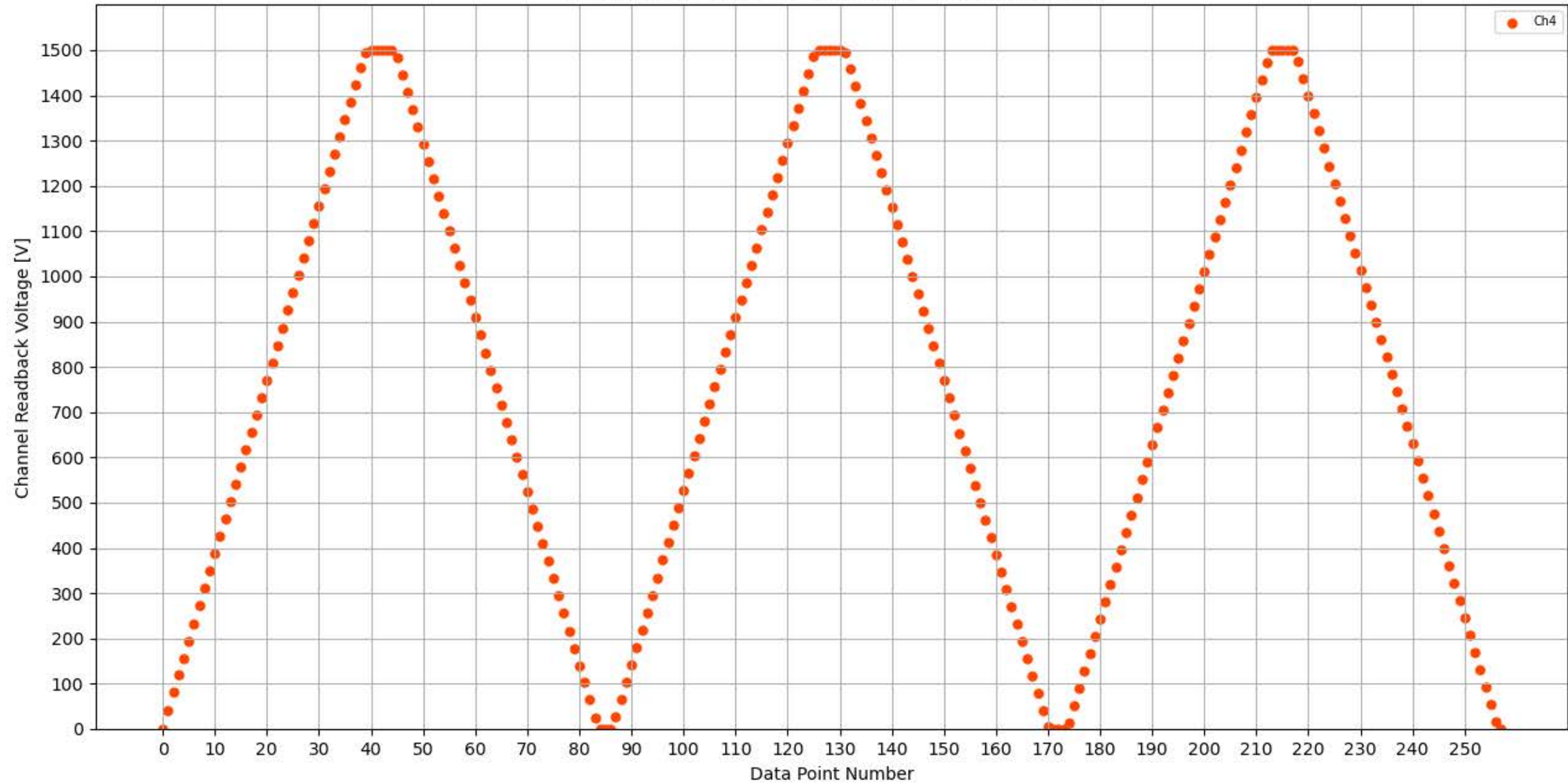
Voltage Ramp Test (Python) Bd #304, Slot #8, Ch #4
