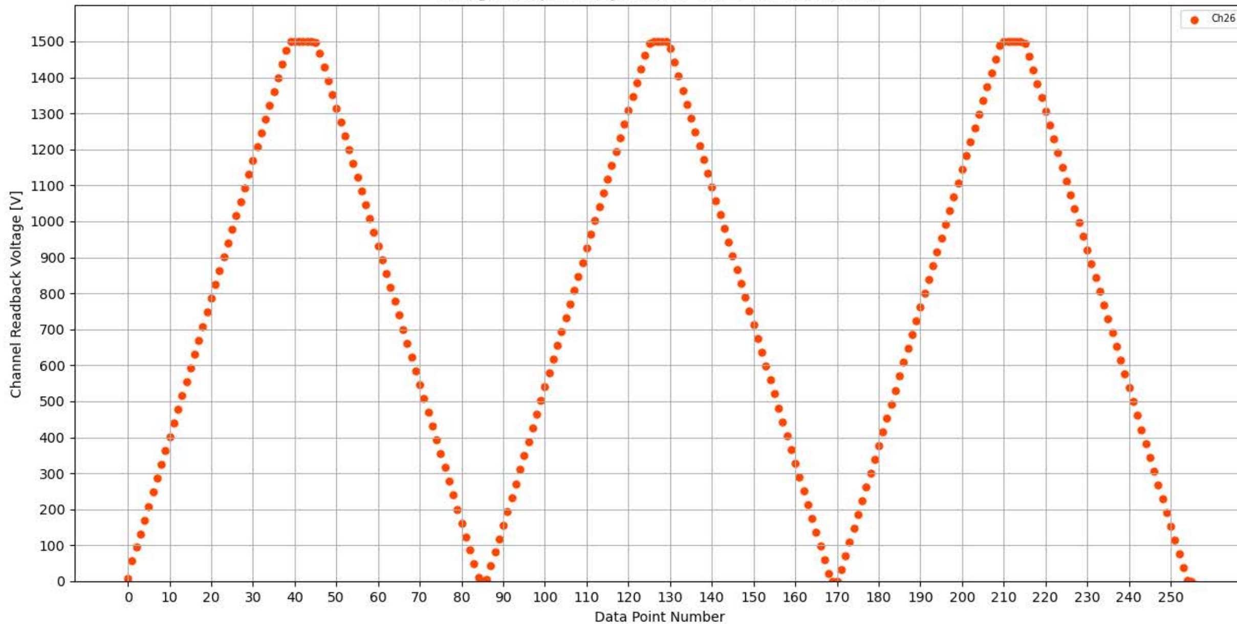
Voltage Ramp Test (Python) Bd #304, Slot #8, Ch #26
