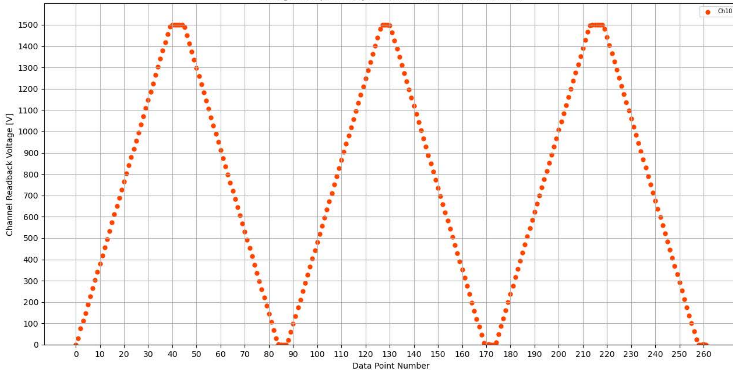
Voltage Ramp Test (Python) Bd #304, Slot #8, Ch #10
