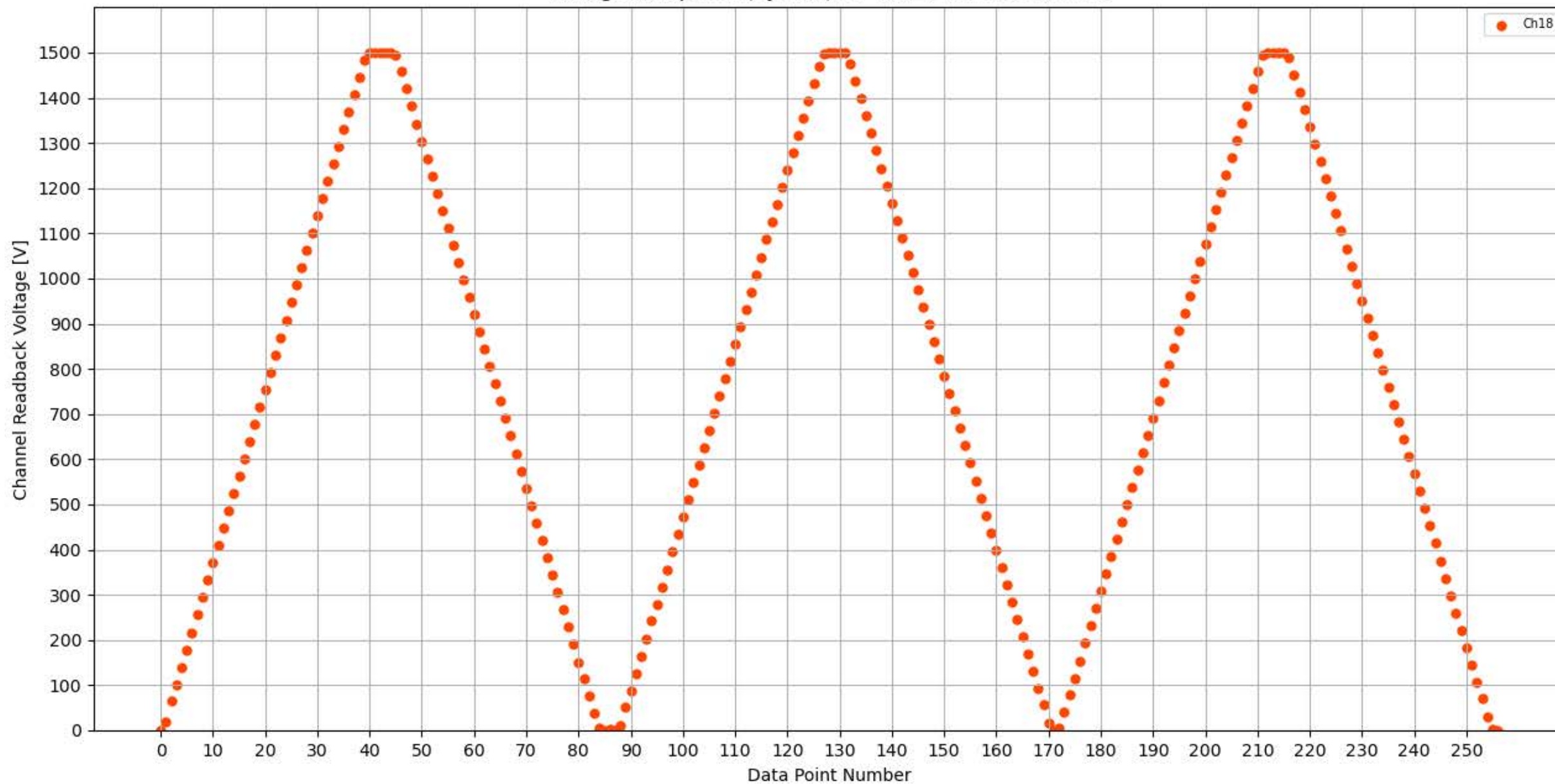
Voltage Ramp Test (Python) Bd #304, Slot #8, Ch #18
