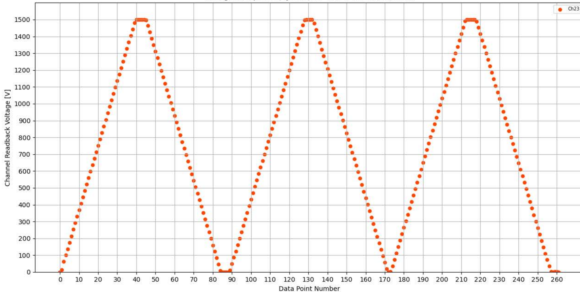
Voltage Ramp Test (Python) Bd #304, Slot #8, Ch #23
