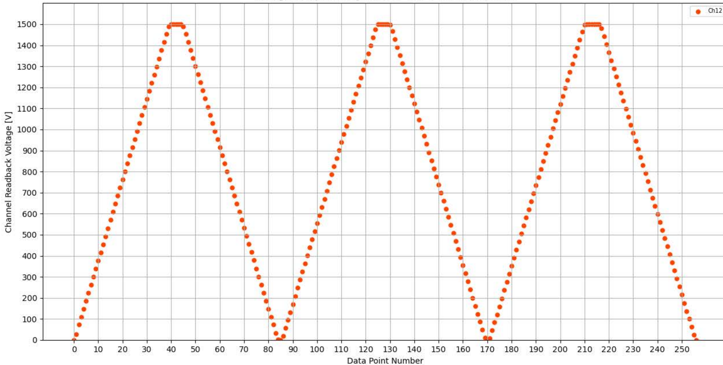
Voltage Ramp Test (Python) Bd #304, Slot #8, Ch #12
