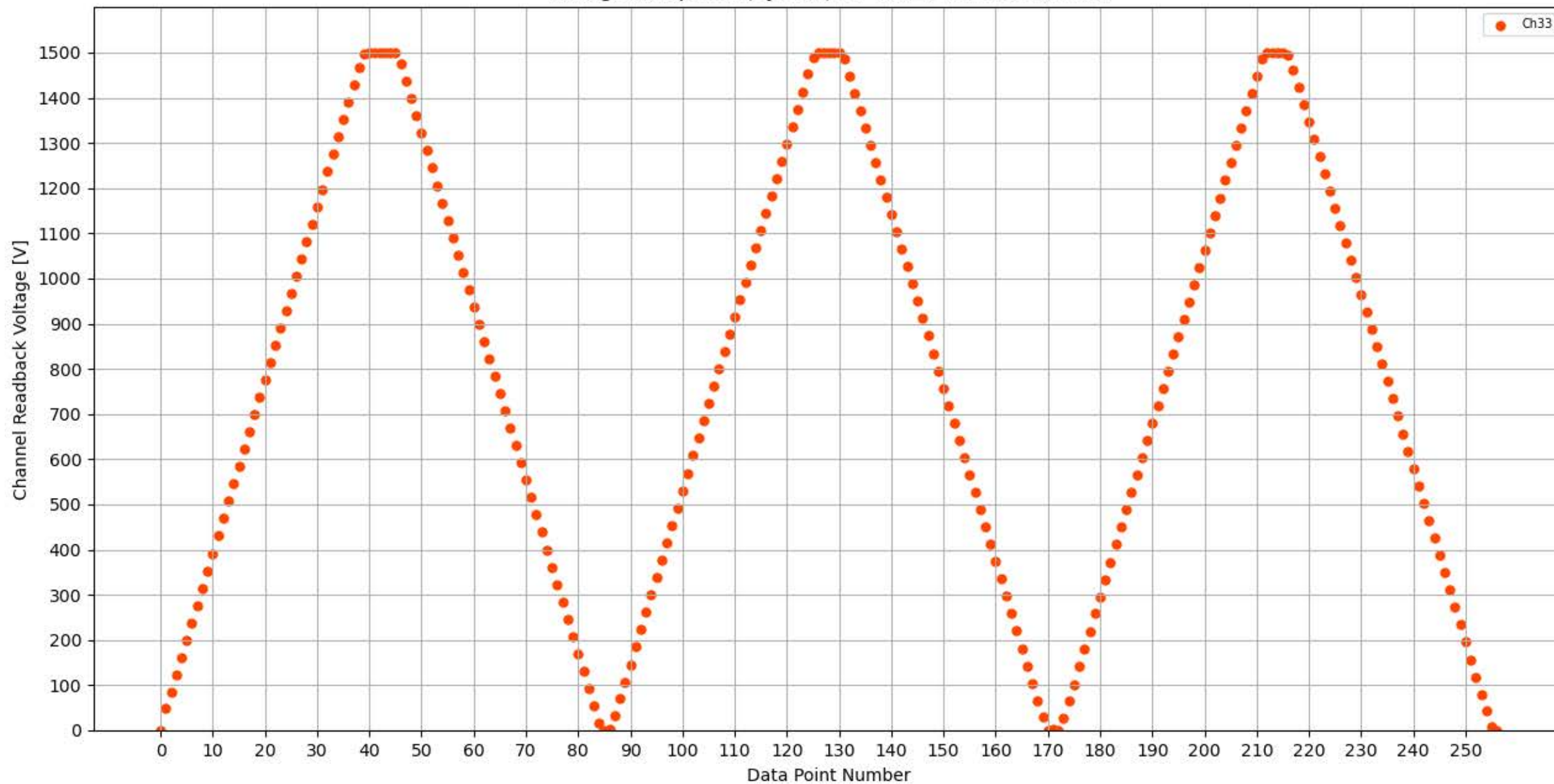
Voltage Ramp Test (Python) Bd #304, Slot #8, Ch #33
