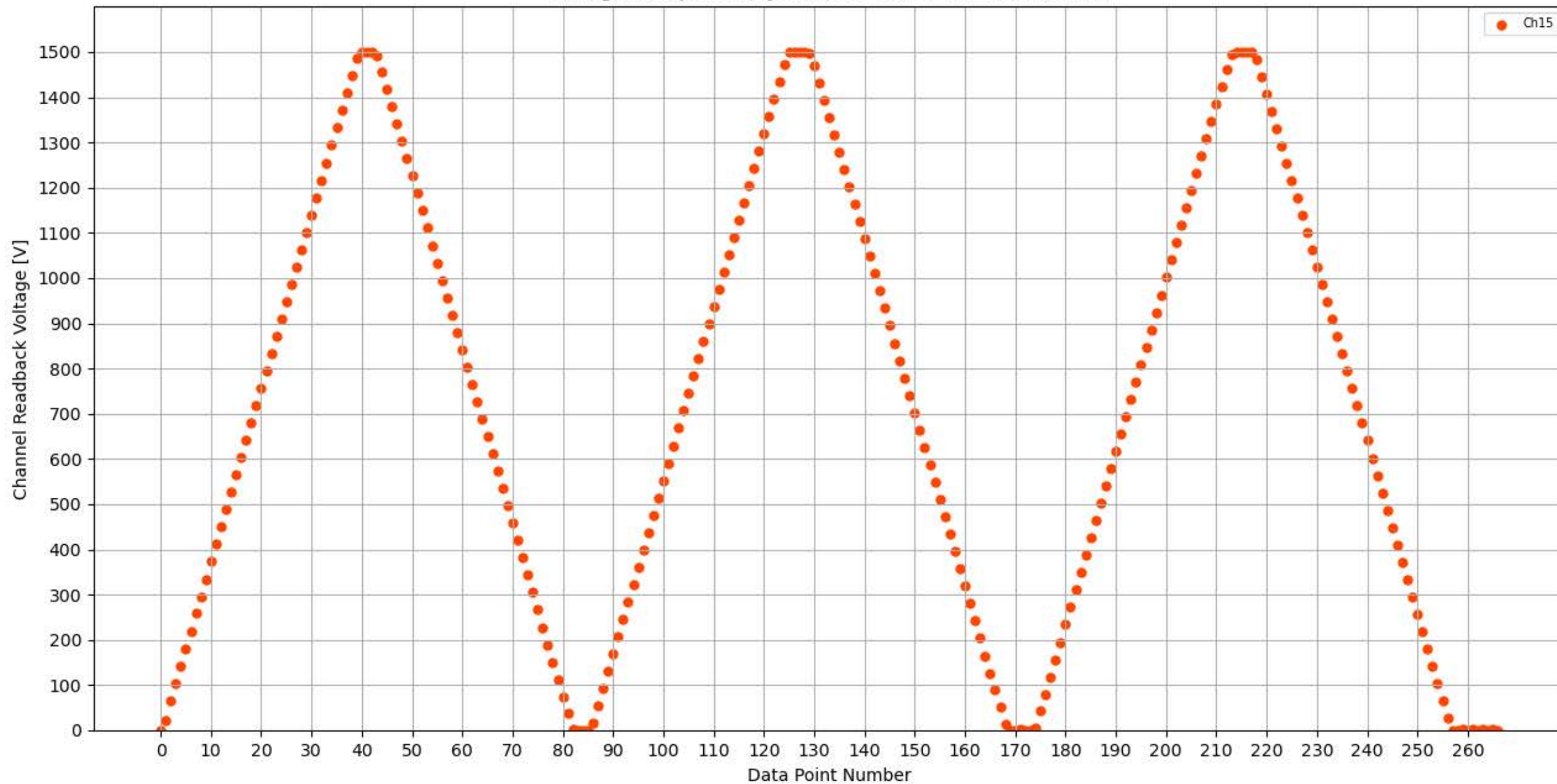
Voltage Ramp Test (Python) Bd #304, Slot #8, Ch #15
