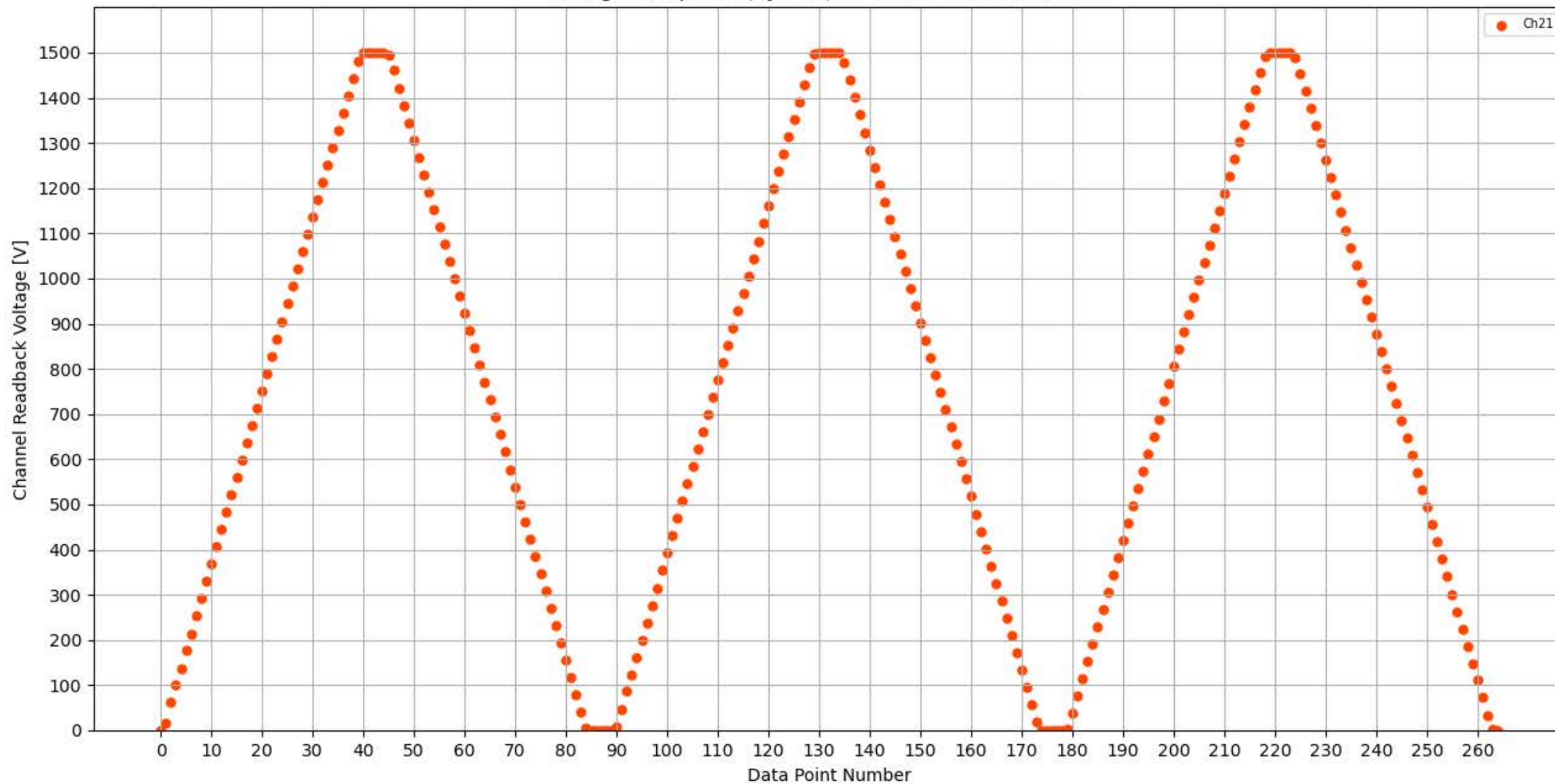
Voltage Ramp Test (Python) Bd #304, Slot #8, Ch #21
