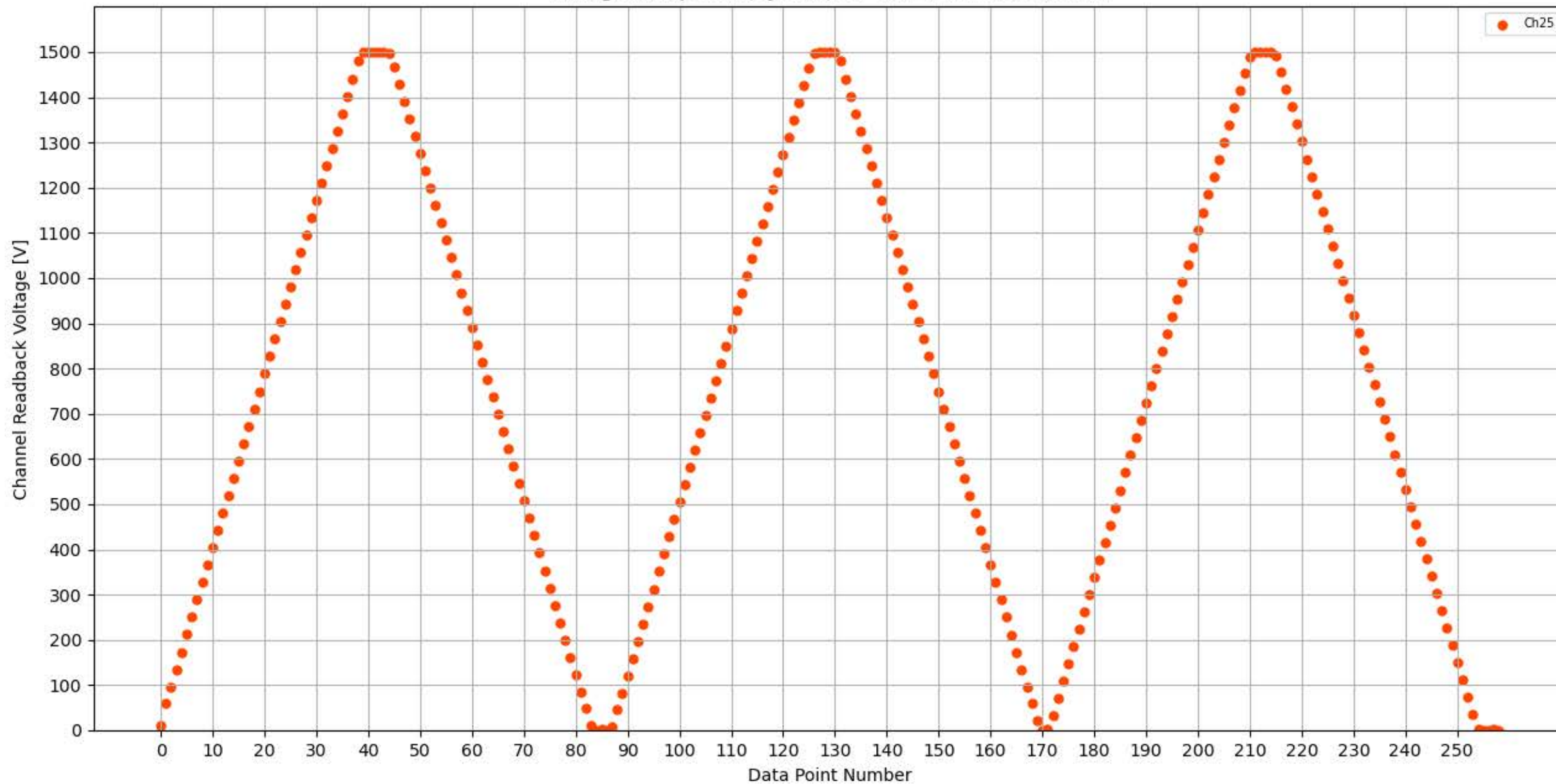
Voltage Ramp Test (Python) Bd #304, Slot #8, Ch #25
