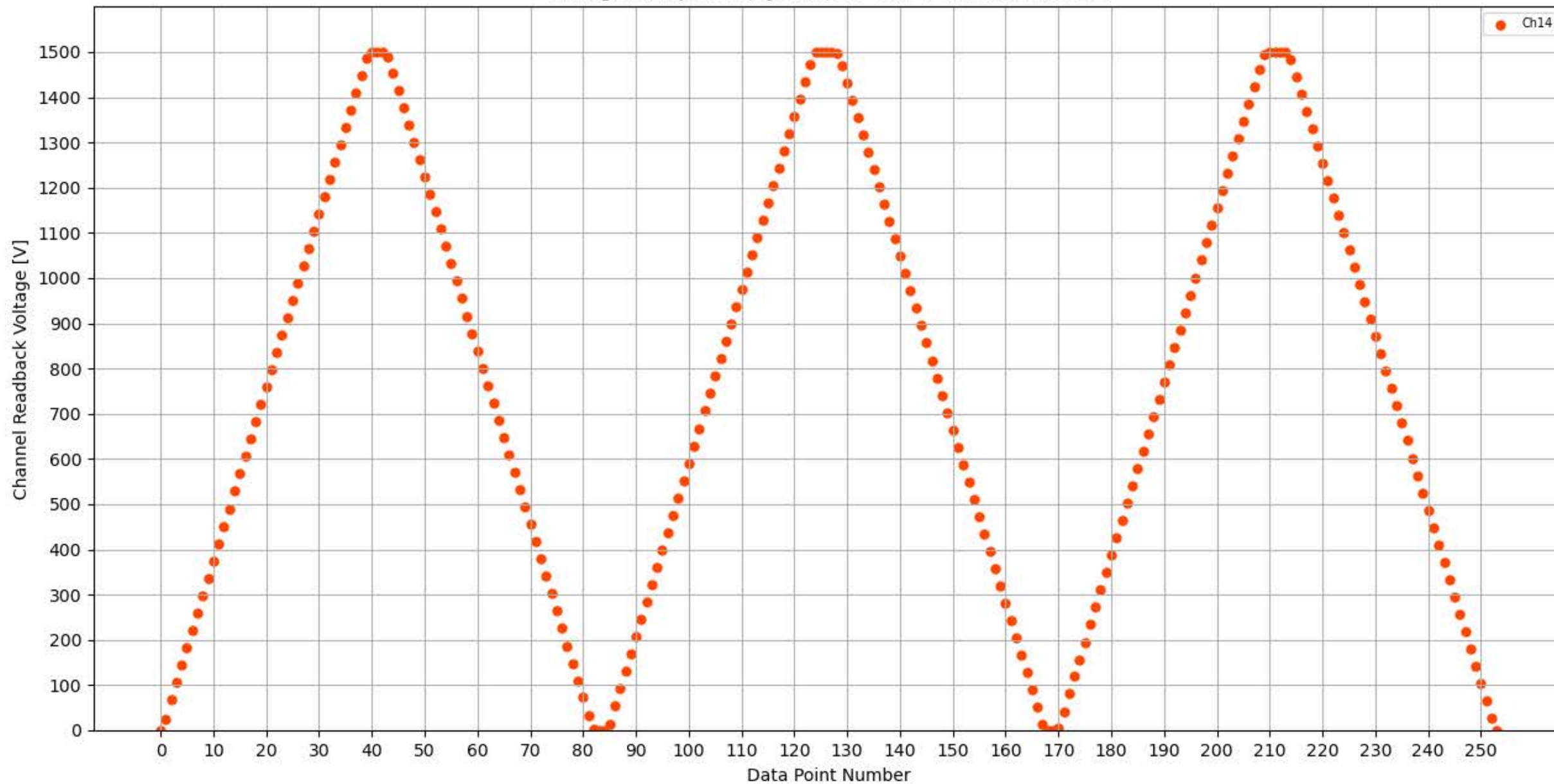
Voltage Ramp Test (Python) Bd #304, Slot #8, Ch #14
