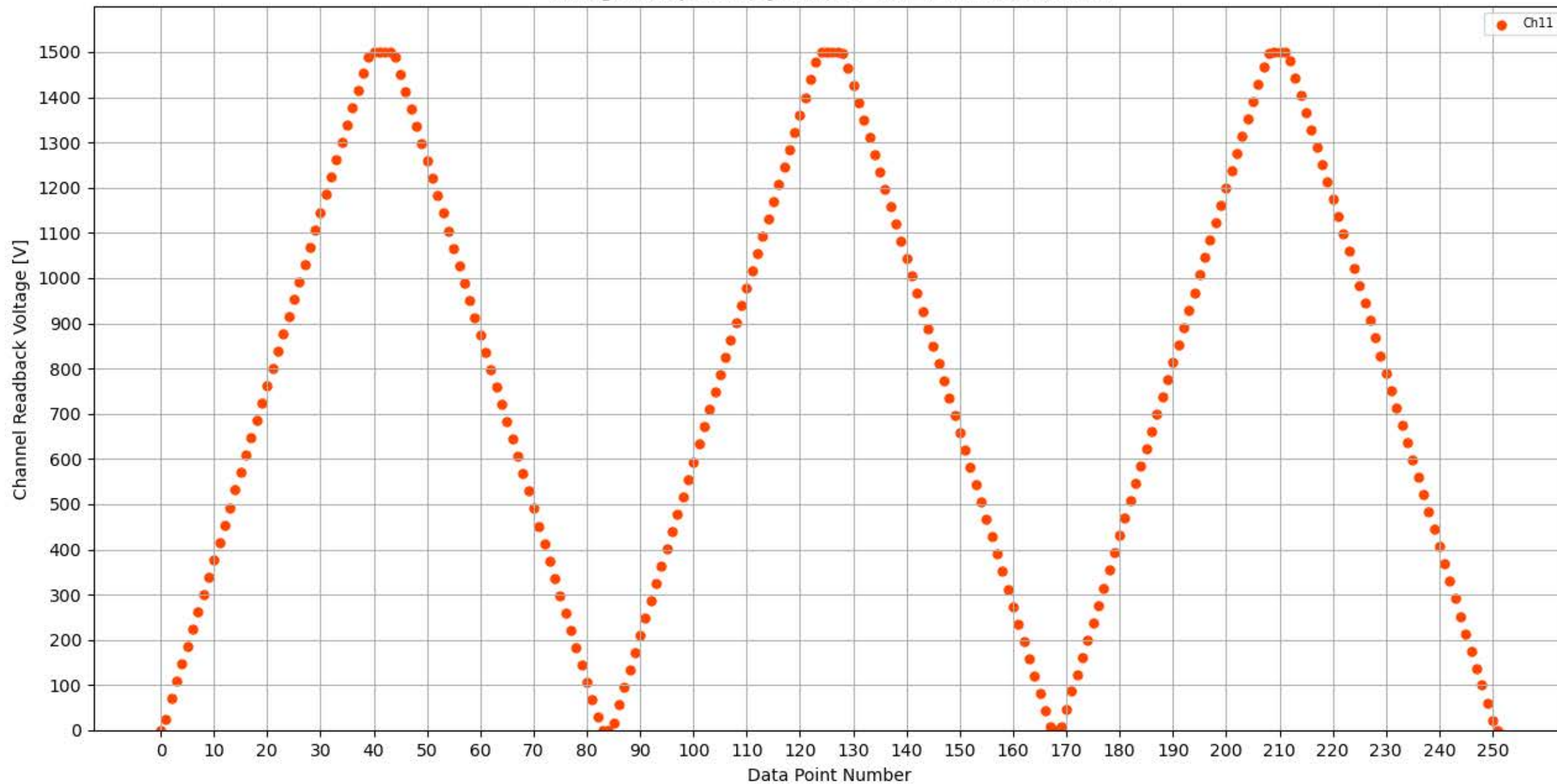
Voltage Ramp Test (Python) Bd #304, Slot #8, Ch #11
