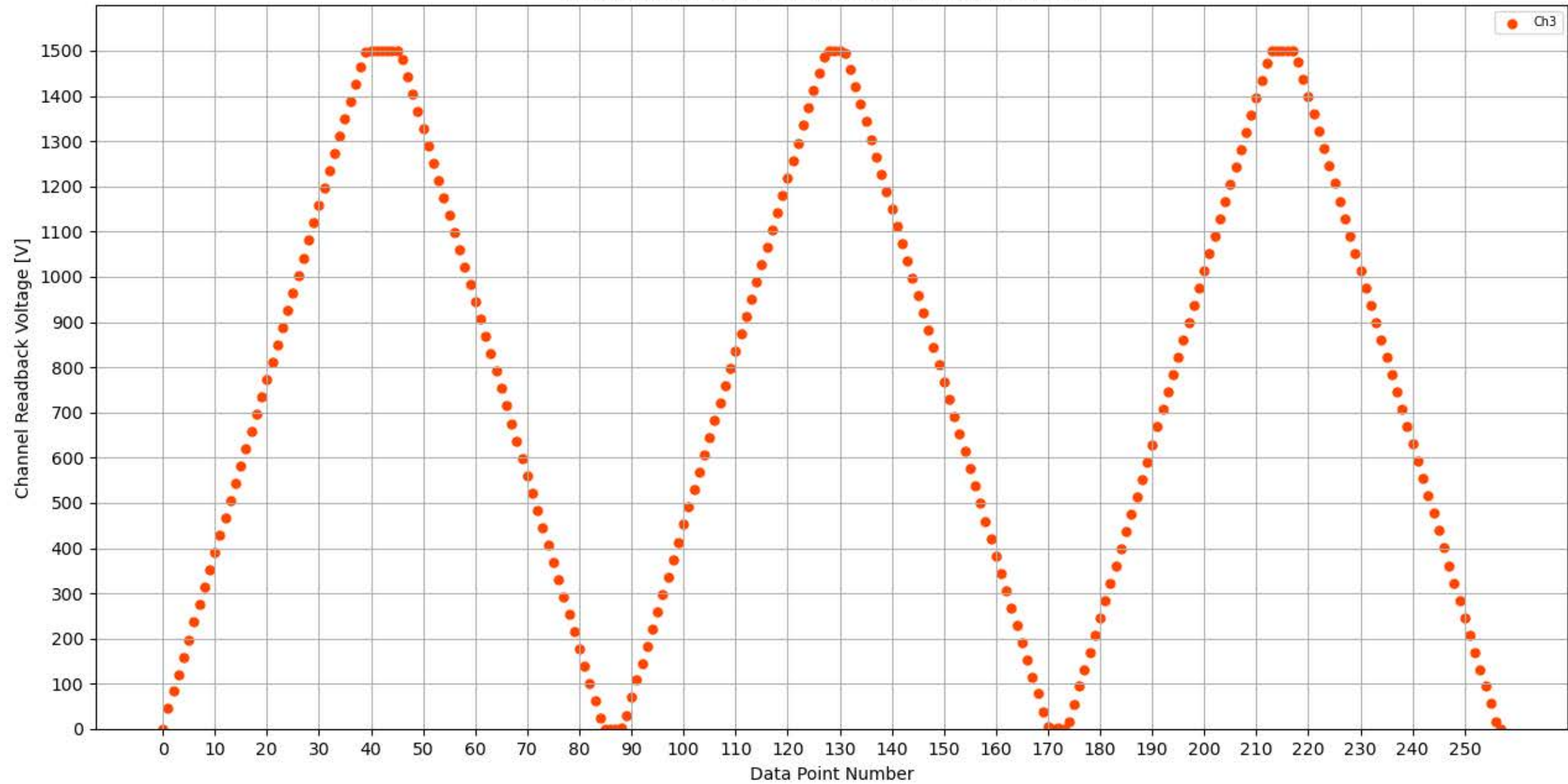
Voltage Ramp Test (Python) Bd #304, Slot #8, Ch #3
