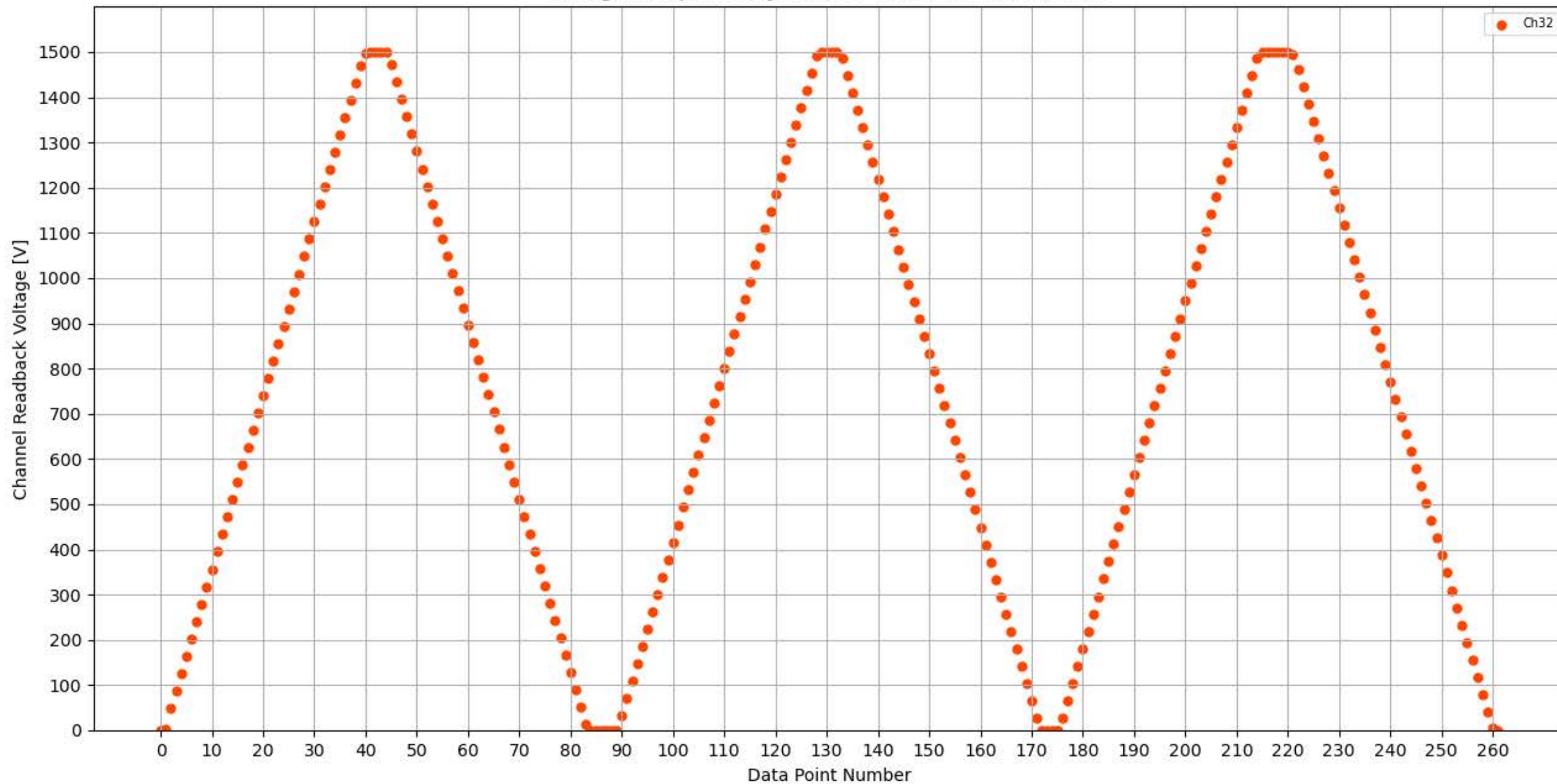
Voltage Ramp Test (Python) Bd #304, Slot #8, Ch #32
