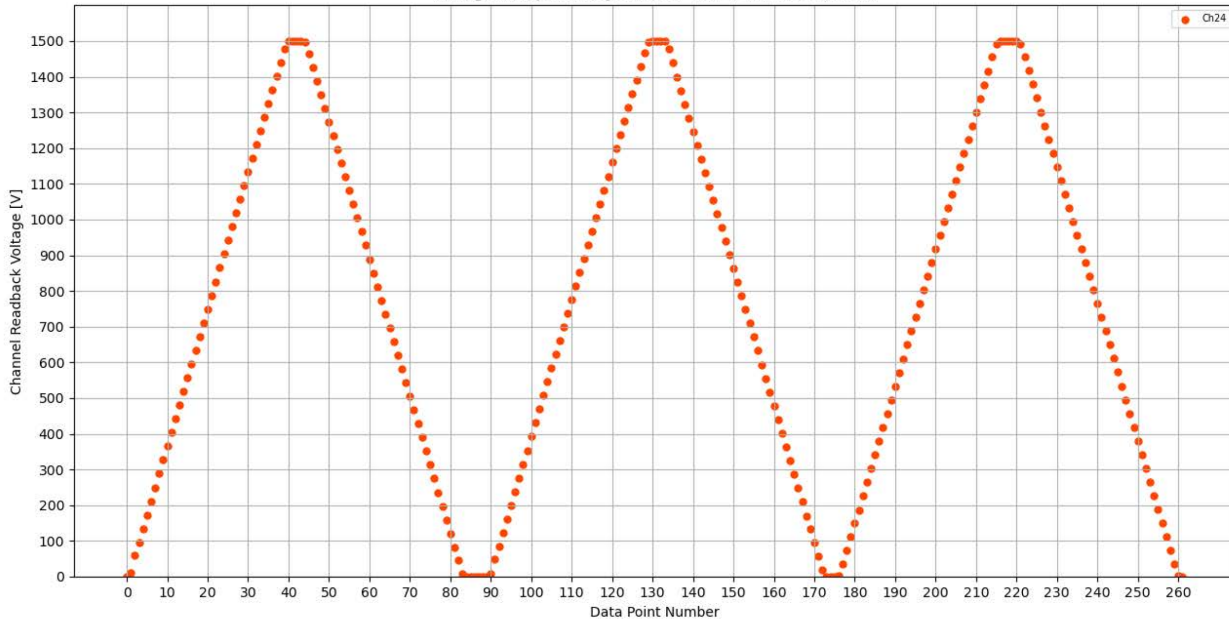
Voltage Ramp Test (Python) Bd #304, Slot #8, Ch #24
