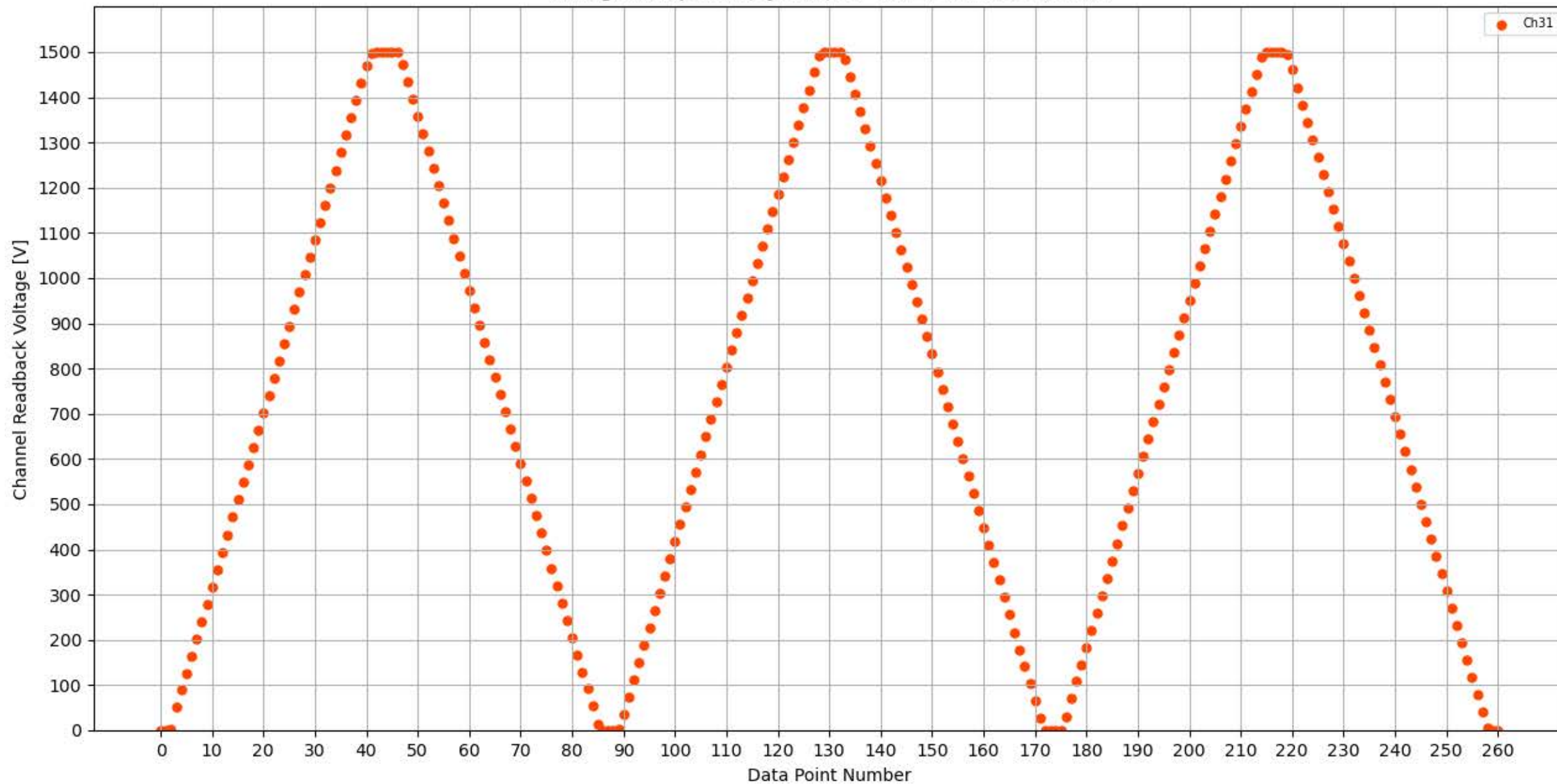
Voltage Ramp Test (Python) Bd #304, Slot #8, Ch #31
