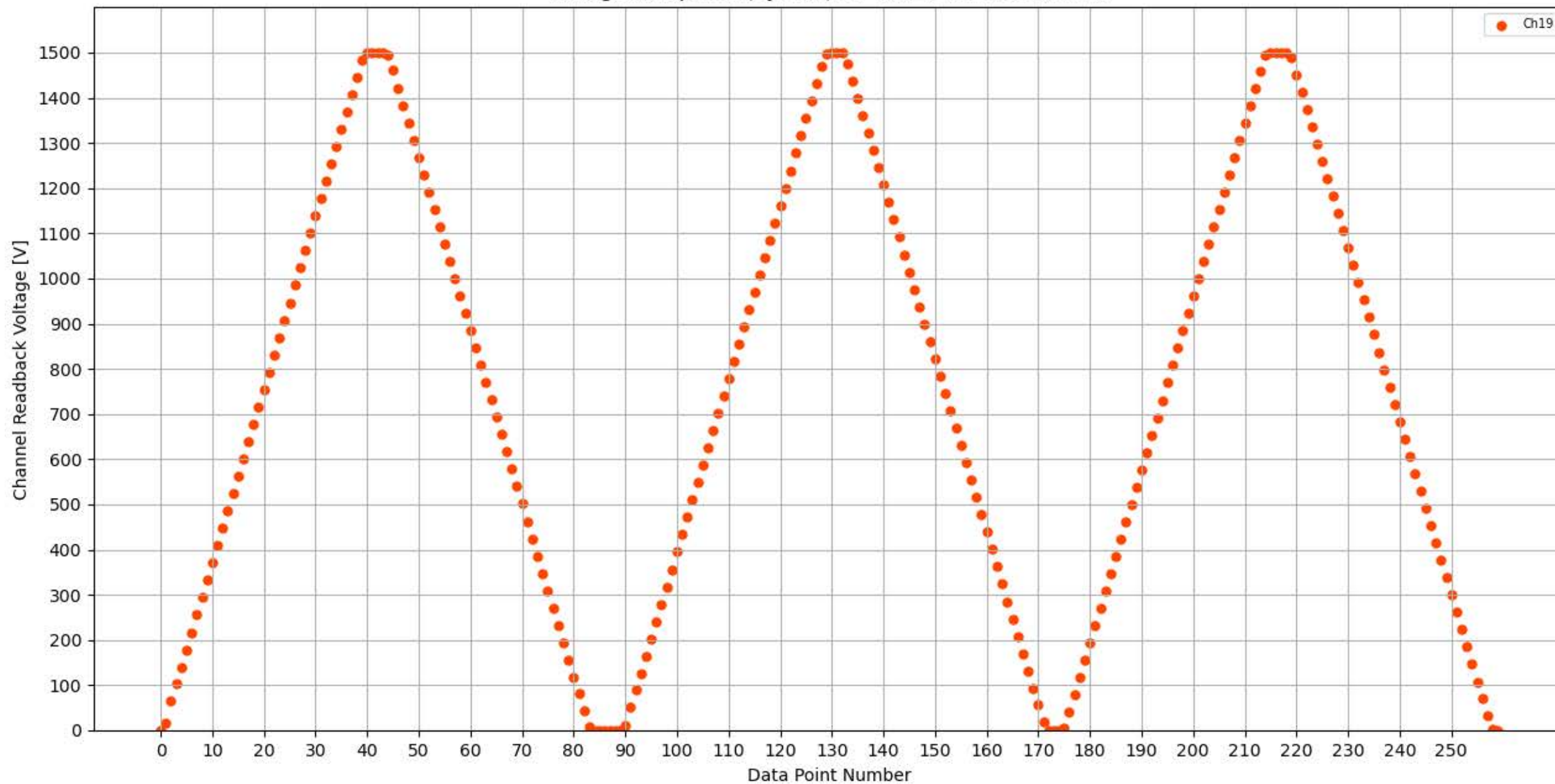
Voltage Ramp Test (Python) Bd #304, Slot #8, Ch #19
