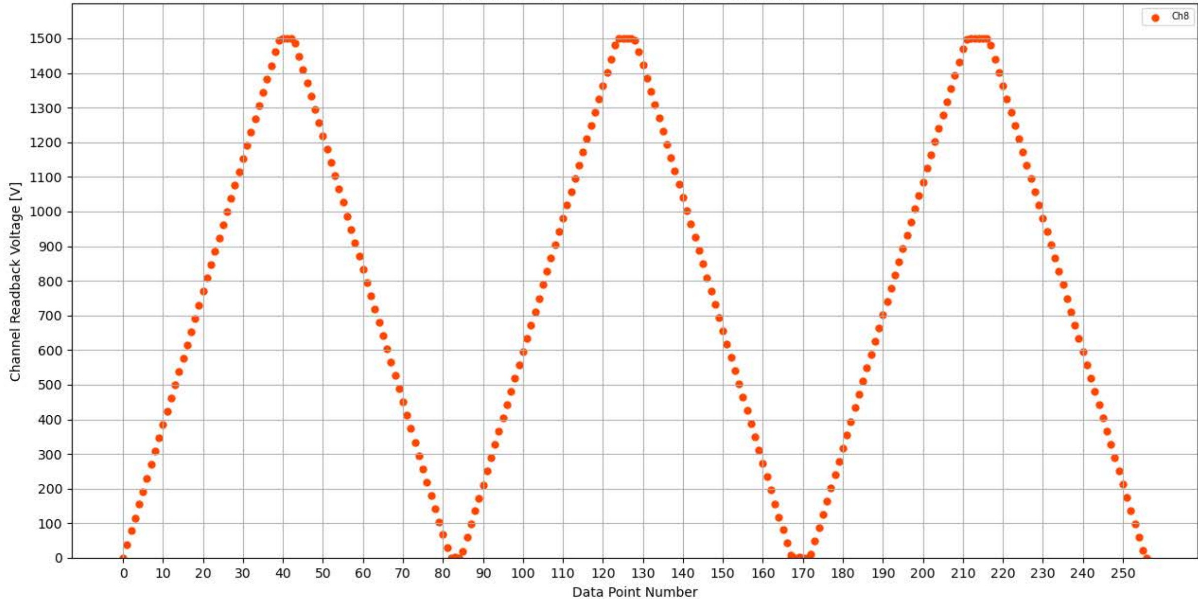
Voltage Ramp Test (Python) Bd #304, Slot #8, Ch #8
