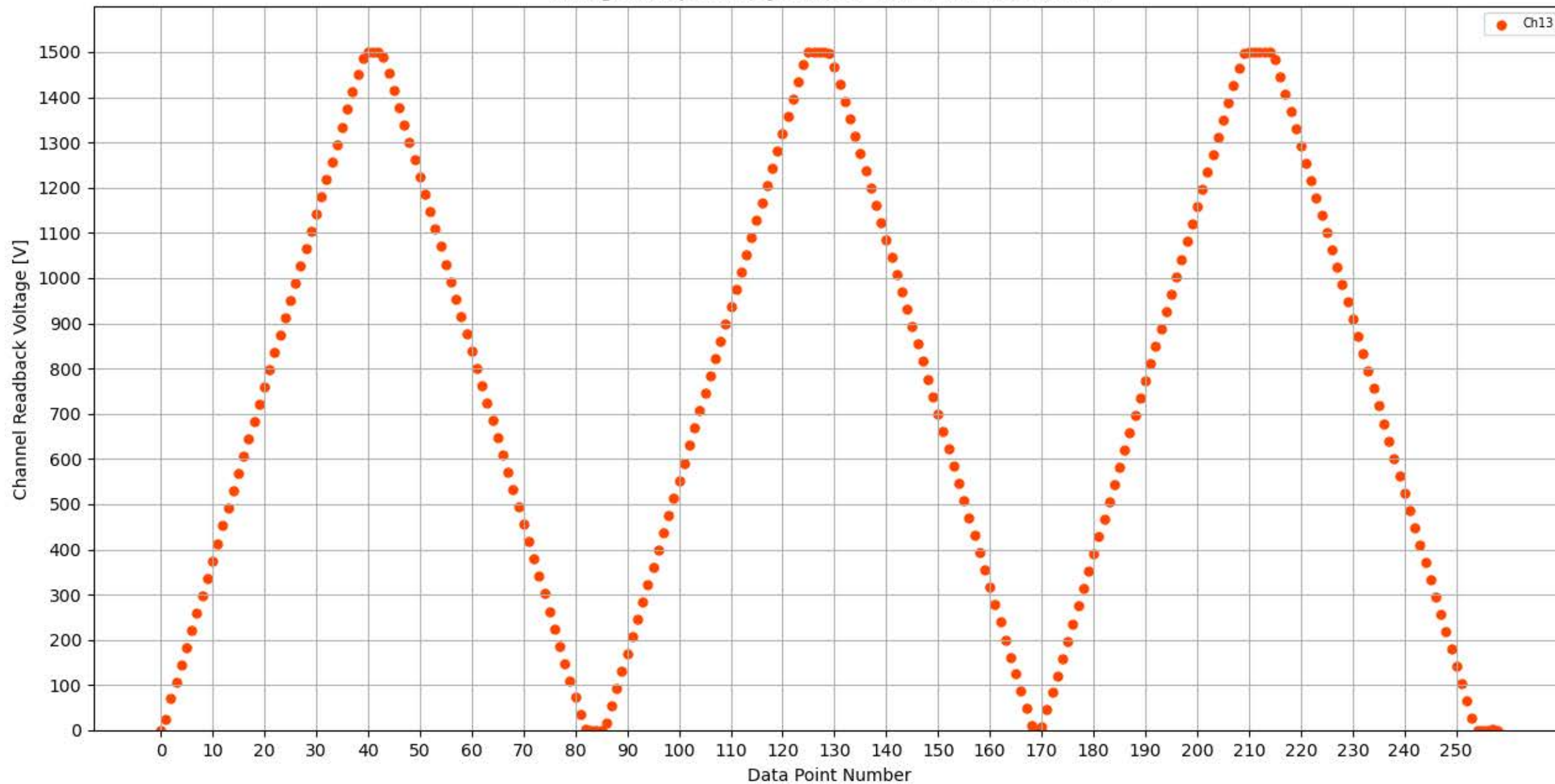
Voltage Ramp Test (Python) Bd #304, Slot #8, Ch #13
