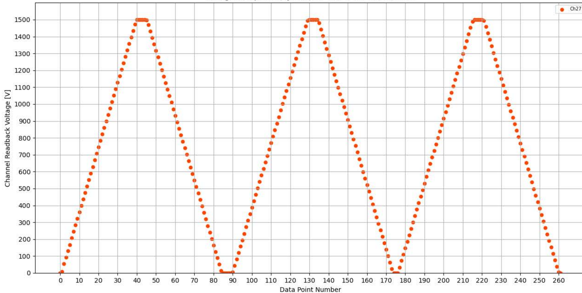
Voltage Ramp Test (Python) Bd #304, Slot #8, Ch #27
