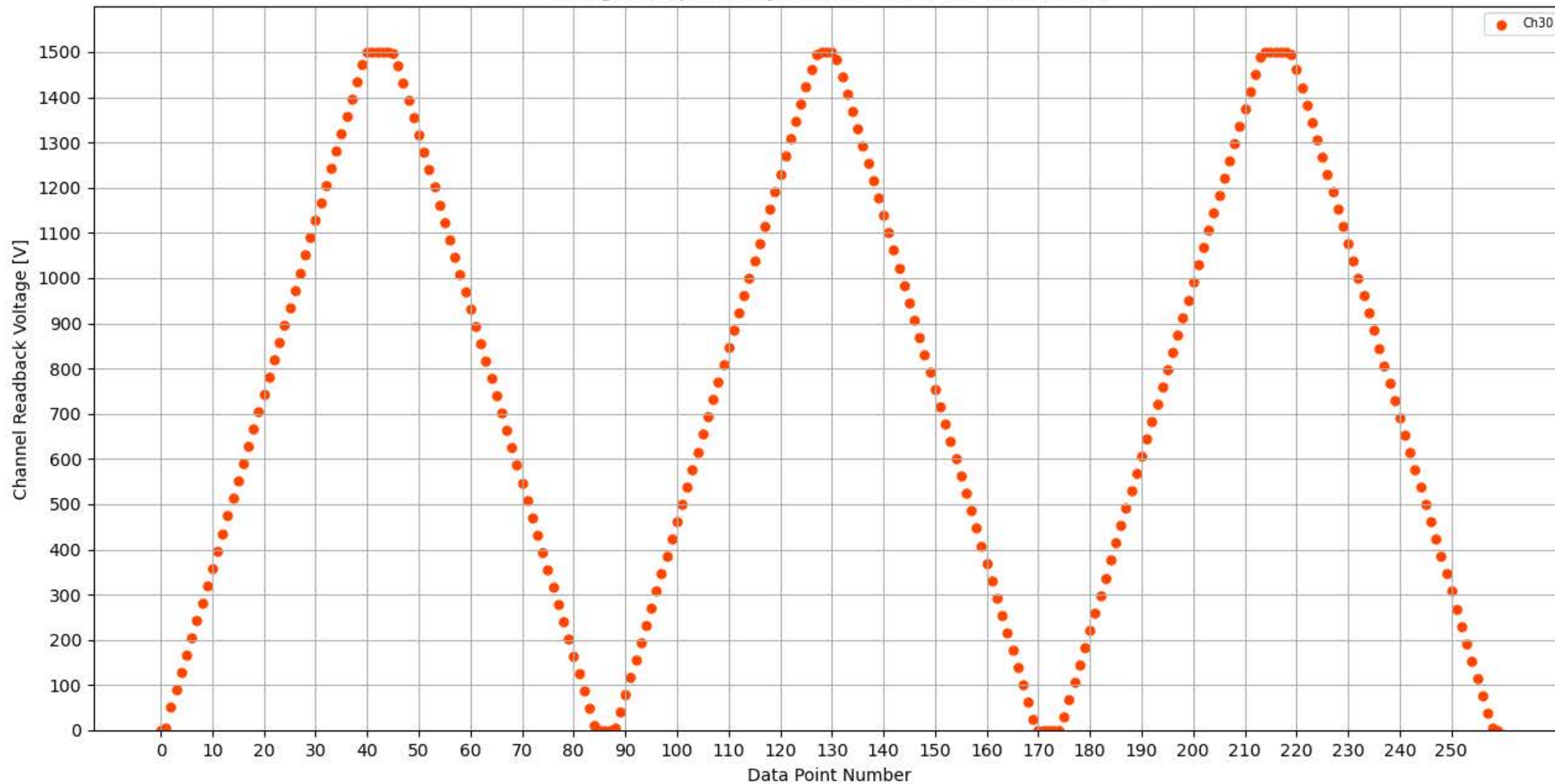
Voltage Ramp Test (Python) Bd #304, Slot #8, Ch #30
