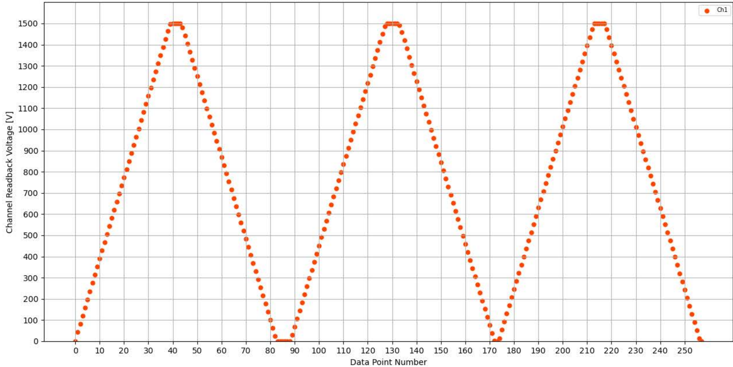
Voltage Ramp Test (Python) Bd #304, Slot #8, Ch #1
