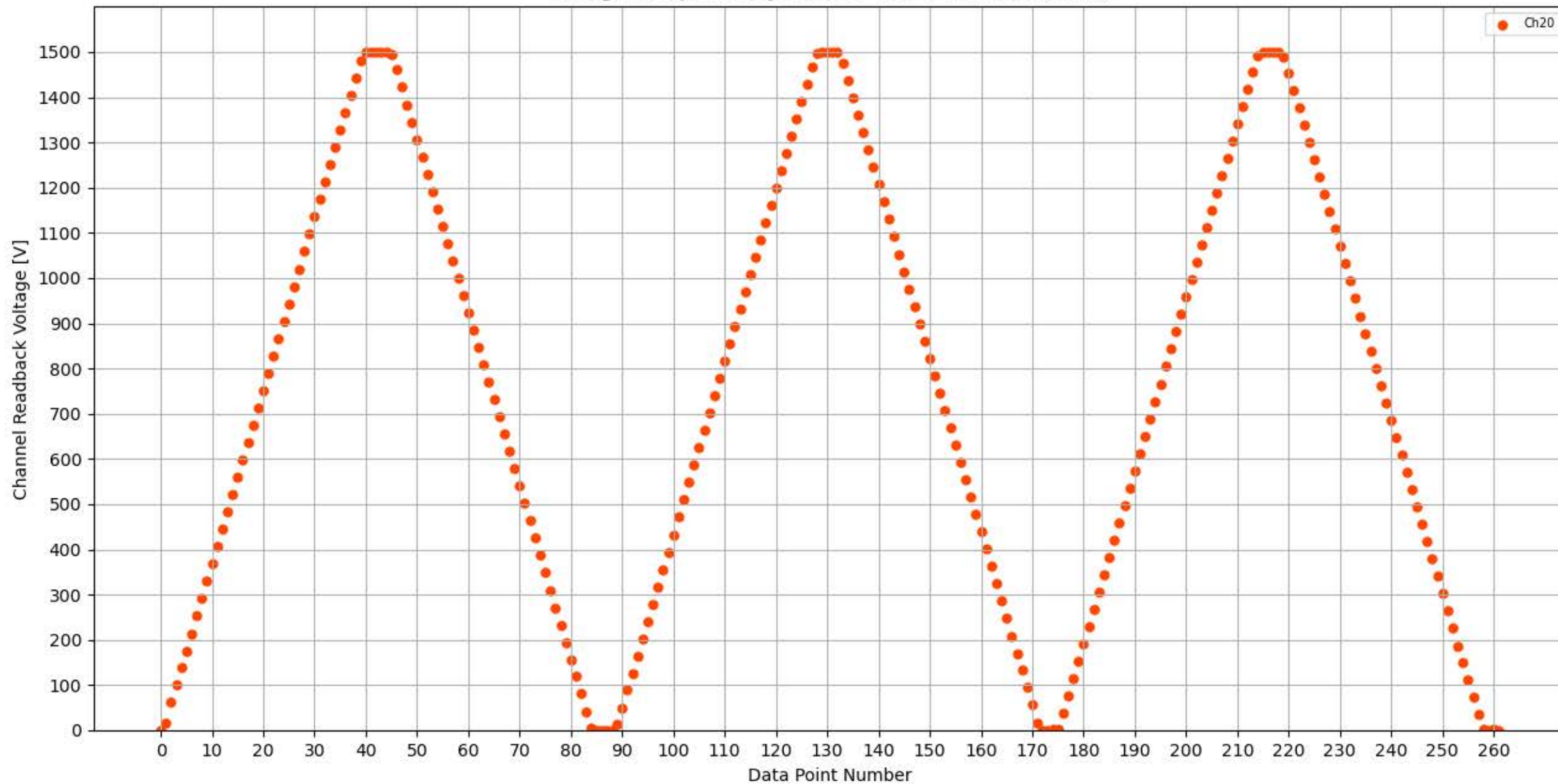
Voltage Ramp Test (Python) Bd #304, Slot #8, Ch #20
