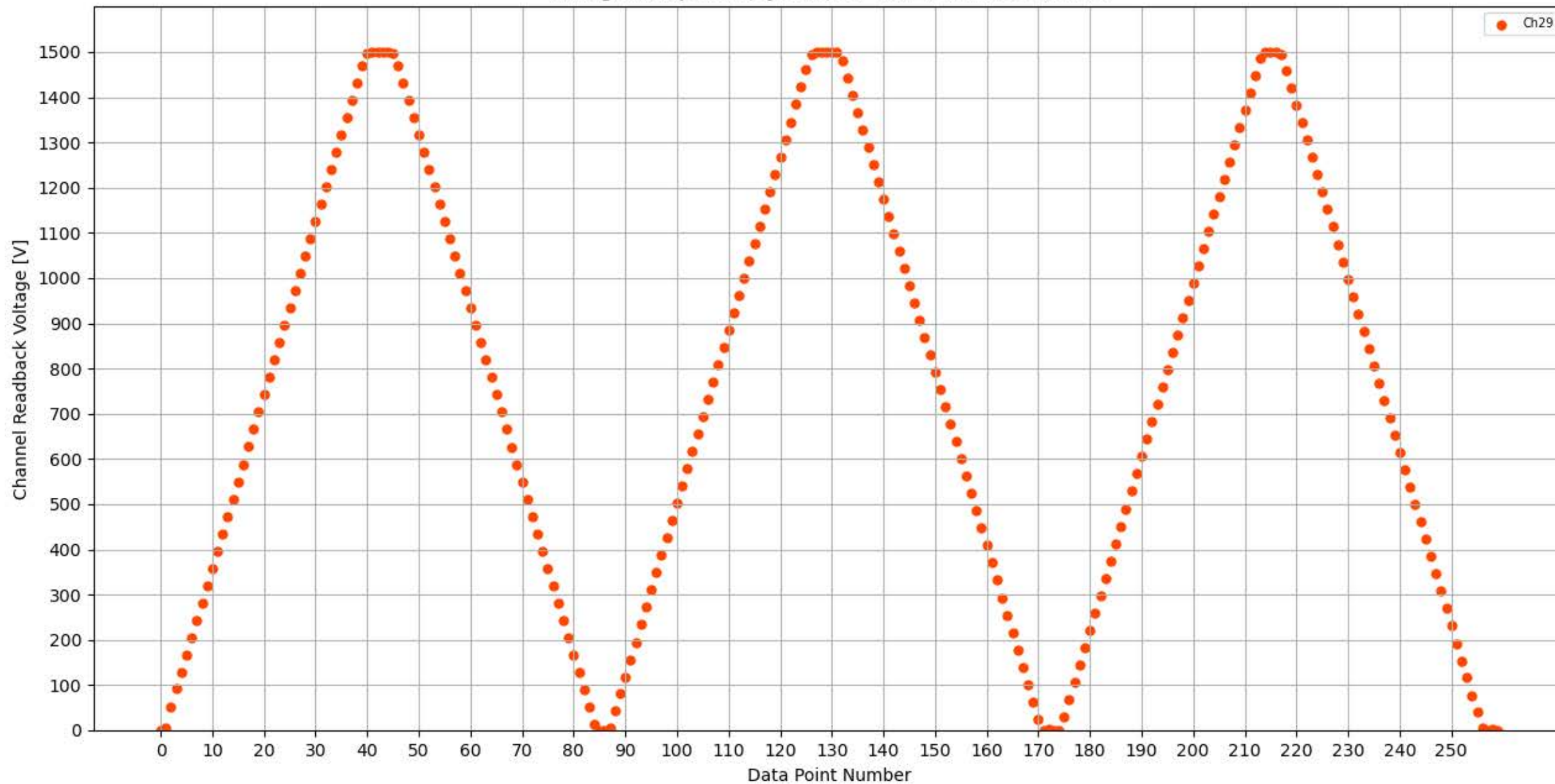
Voltage Ramp Test (Python) Bd #304, Slot #8, Ch #29
